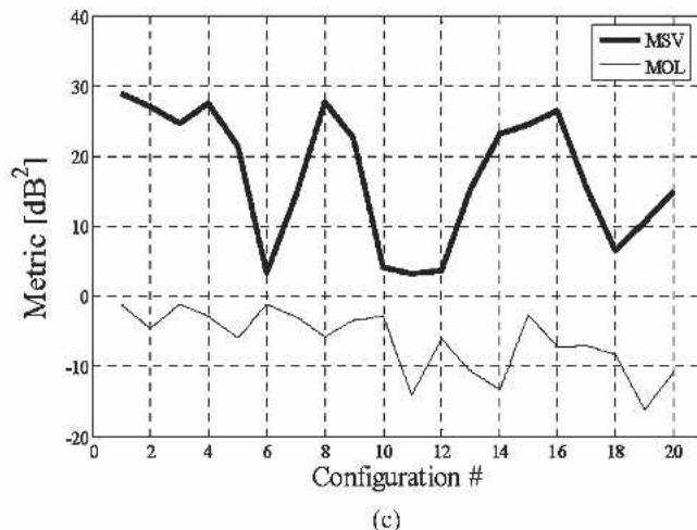
Fig. 5. (a) “Practical” subwoofer configurations in virtual test room (absorption coefficient 0.05). (b) Subwoofer and seat locations. (c) MSV and MOL metrics for all configurations. Note that MOL in (c) is normalized for number of subwoofers used (correction factor -20 \log(N) ). Correction only to this graph.
